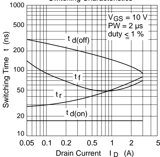
Switching Characteristics
